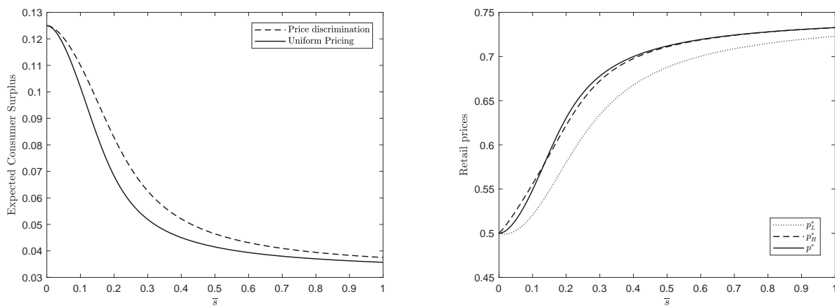
Figure 8: N = 3 and D(p) = 1 - p . Left: Expected Consumer Surplus for different values of \bar{s} . Right: Retail Prices for different values of \bar{s} .
