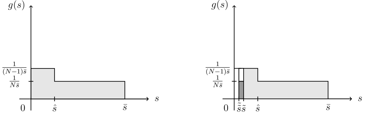
Figure 9: Left: Search cost compositions of demand for a low cost retailer. Right: Share of consumers that buy at the deviating low cost retailer; where s \sim U[0, \bar{s}] .
