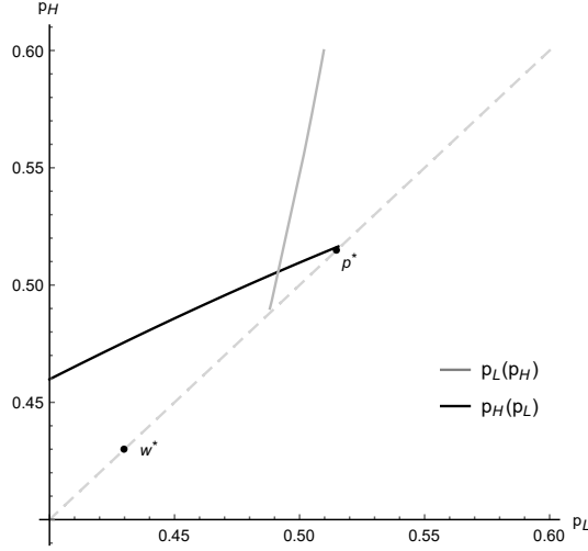
Figure 4: Retailers' behaviour for marginal deviations from uniform wholesale prices, when \bar{s} = 0.05 , w^* = 0.4299 and p^* = 0.5149
