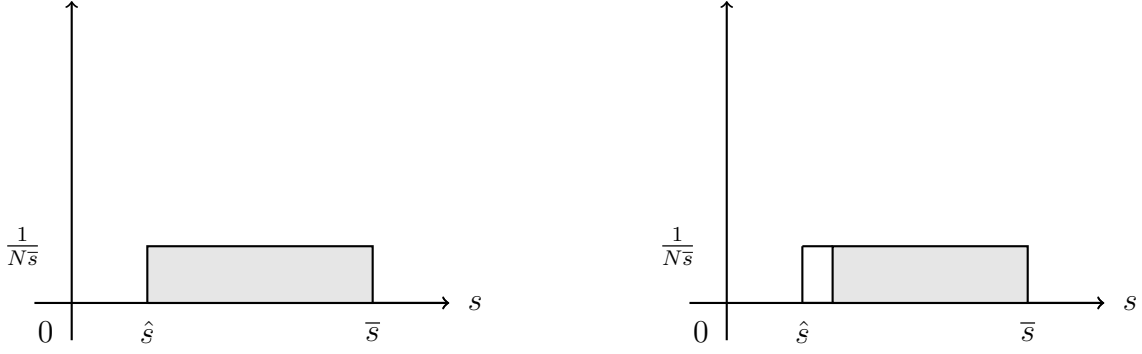
Figure 2: Left: Search cost compositions of demand for a high cost retailer. Right: Share of consumers that buy at the deviating high cost retailer.
