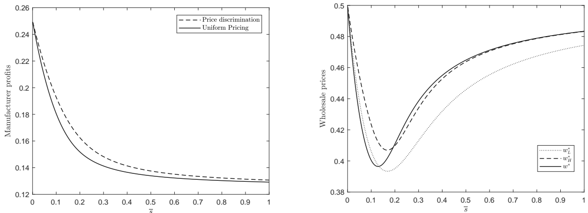
Figure 6: N = 3 and D(p) = 1 - p . Left: Manufacturer's profit for different values of \bar{s} . Right: Wholesale prices for different values of \bar{s} .
