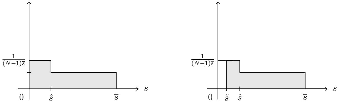
Figure 3: Left: Search cost compositions of demand for a low cost retailer. Right: Share of consumers that buy at the deviating low cost retailer.
