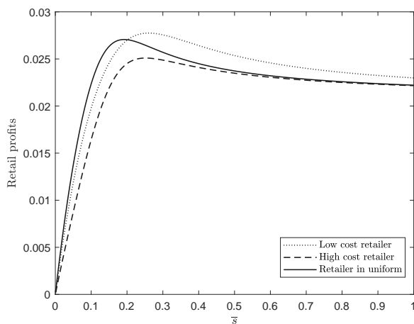
Figure 7: Retailer Profits for different values of \bar{s} , when N = 3 and D(p) = 1 - p .
